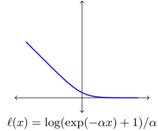
Fig. 1. Continuous hinge loss
